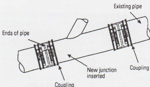
Figure 22 - Insertion of junction
