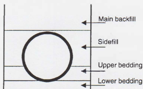
Figure 1 - Pipe trench installation
