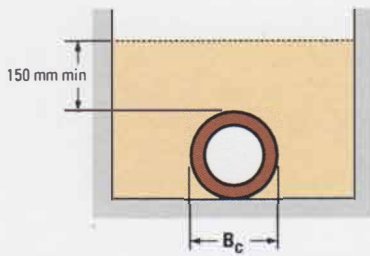
Figure 5 - Class D - Trimmed trench bottom Bedding factor 1.1 (Ref. 14)
