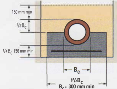
Figure 12 - Reinforced concrete bed Bedding factor 3.4 (0.4 % steel) (Refs. 27 & 28)
