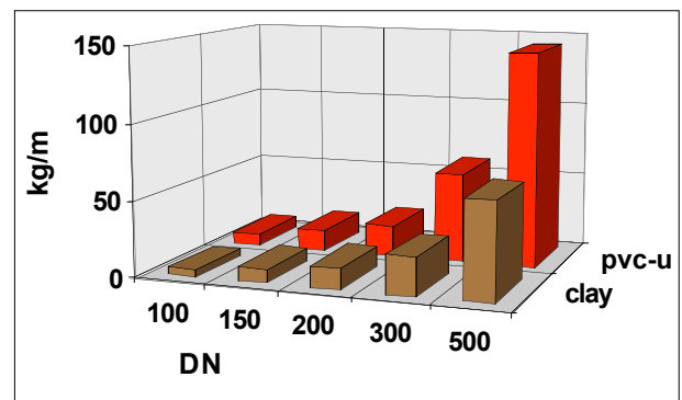
Fig. 1 : Carbon dioxide emission in pipe production
